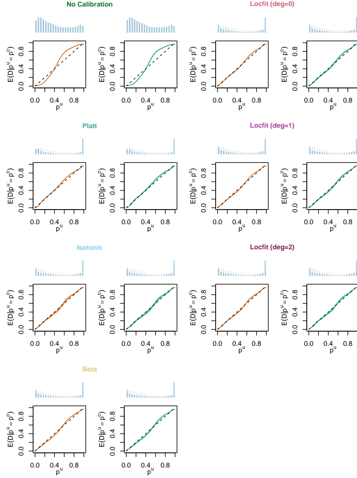
Figure 20: Calibration Curves Obtained with Local Regression , for the Classification Random Forest, for the Calibration Set and for the Test Set . The curves are the averages values obtained on 200 different splits of the calibration and test datasets, and the color bands are the 95% bootstrap confidence intervals. The histogram on top of each graph show the distribution of the uncalibrated scores, and that of the calibrated scores.
