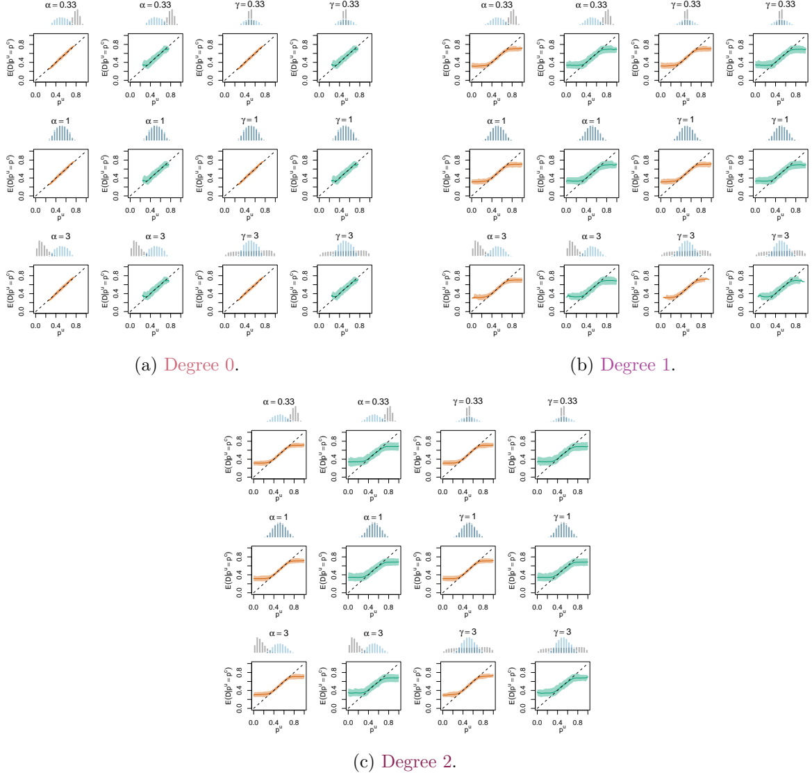
Figure 16: Calibration Curves Calculated with Scores Recalibrated Using Local Regression with Degree 0 (Panel a), Degree 1 (Panel b), or with Degree 2 (Panel c). The curves are obtained with local regression , for the calibration set (orange) and for the test set (green) for varying values of \alpha and \gamma . The curves are the average values obtained on 200 replications of the simulations, the bands correspond to 95% bootstrap intervals. The histogram on top of each graph show the distribution of the uncalibrated scores , and that of the calibrated scores .
